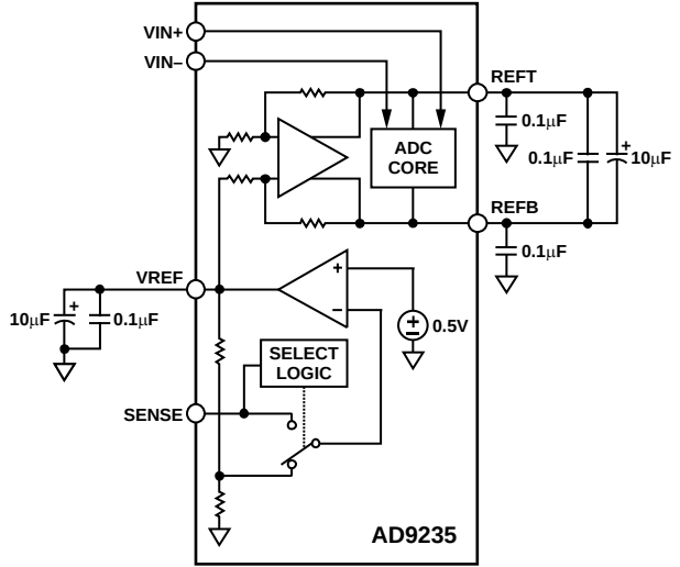
Figure 39. Internal Reference Configuration
