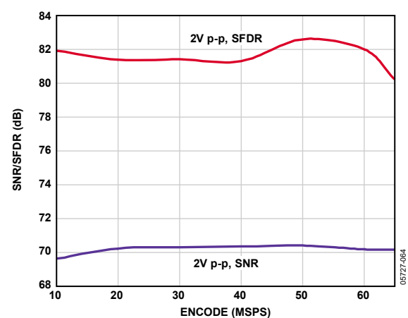
Figure 26. SNR/SFDR vs. Encode, f_{IN} = 35 MHz, f_{SAMPLE} = 65 MSPS
