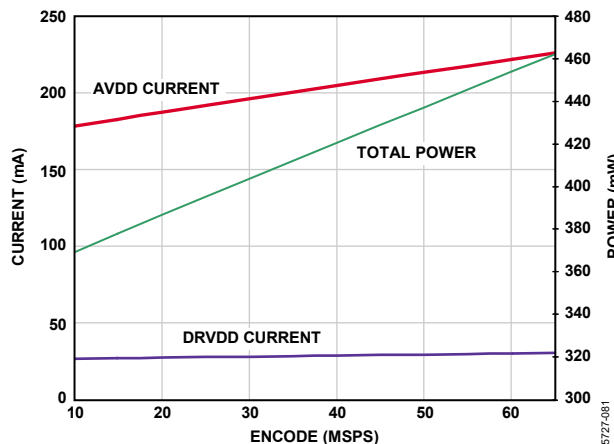
Figure 59. Supply Current vs. f_{\text{SAMPLE}} for f_{\text{IN}} = 10.3 \text{ MHz} , f_{\text{SAMPLE}} = 65 \text{ MSPS}
