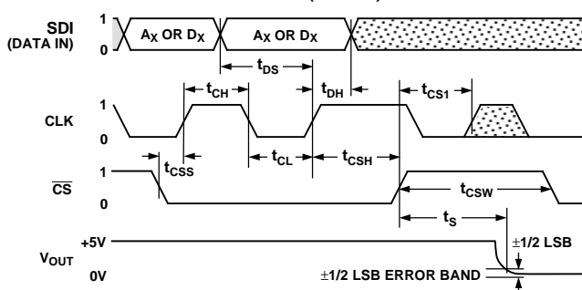
DETAIL SERIAL DATA INPUT TIMING ( \overline{RS} = "1" )
