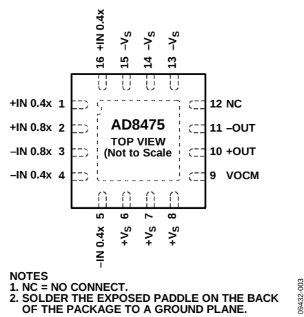
Figure 3. 16-Lead LFCSP Pin Configuration
