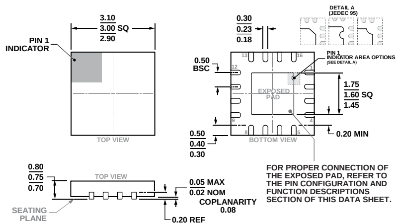
Figure 57. 16-Lead Lead Frame Chip Scale Package [LFCSP] 3 mm × 3 mm Body and 0.75 mm Package Height (CP-16-22)
