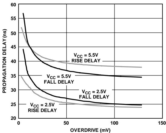
Figure 5. Propagation Delay vs. Input Overdrive, V_{CC} = 2.5\text{ V} and 5.5\text{ V}
