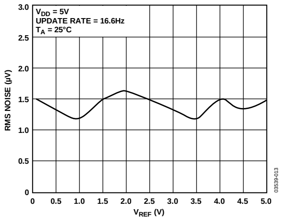
Figure 9. AD7788/AD7789 Noise vs. V_{REF}
