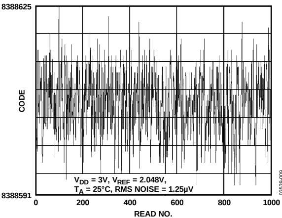
Figure 8. AD7789 Noise Plot
