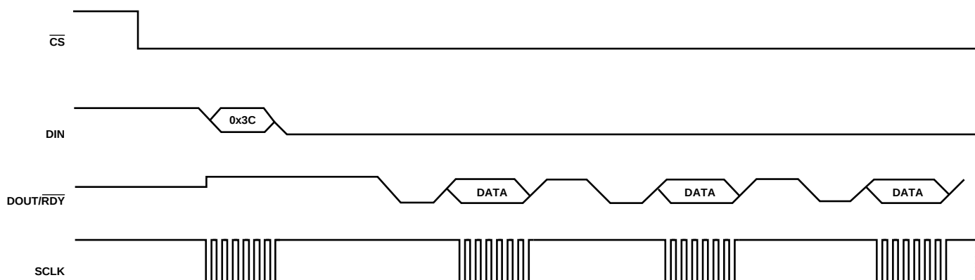
Figure 13. Continuous-Read Mode
