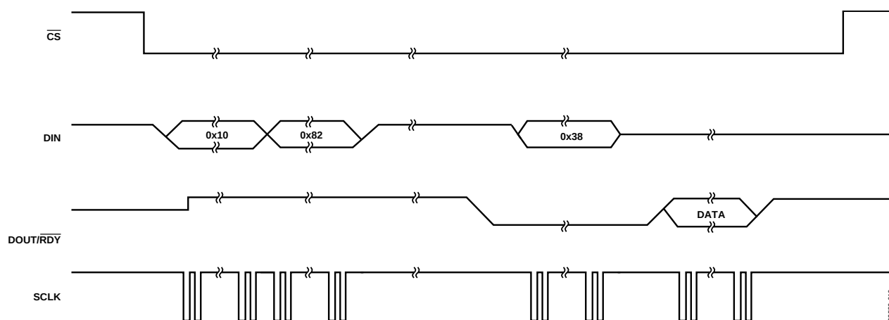
Figure 11. Single Conversion
