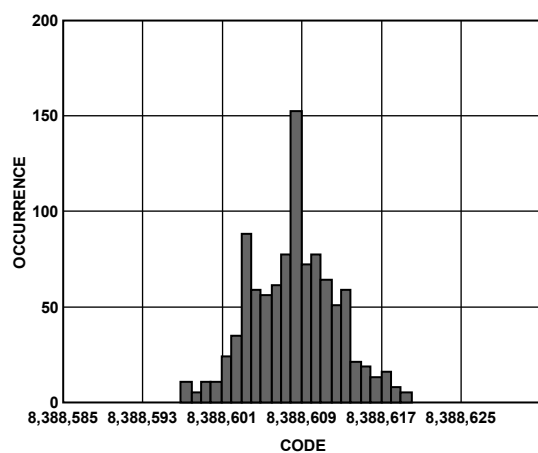
Figure 13. Noise Distribution Histogram ( V_{REF} = AV_{DD} , Update Rate = 16.7 Hz, Gain = 1)
