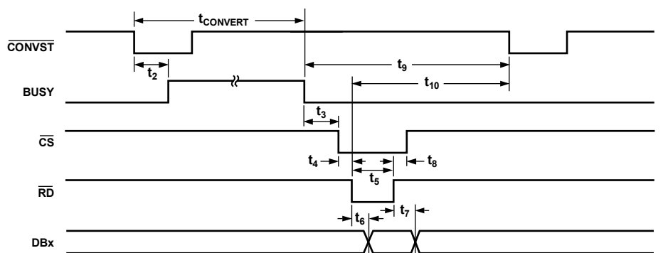
Figure 19. Parallel Port Timing
