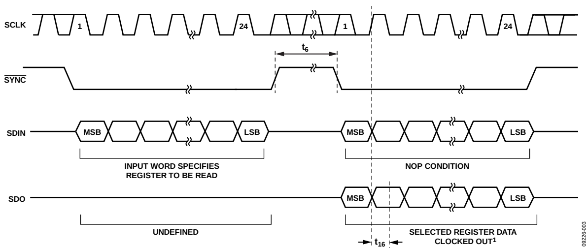
Figure 4. Readback Timing Diagram (Packet Error Checking Disabled)
