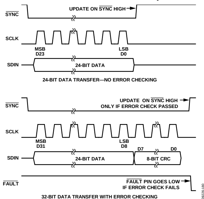
Figure 79. PEC Timing
