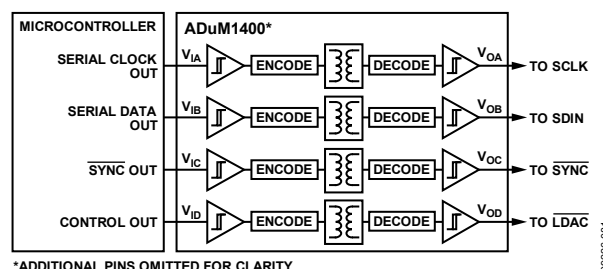
Figure 89. Isolated Interface
