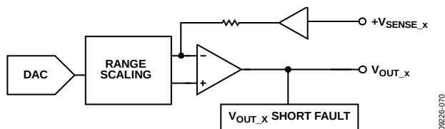
Figure 73. Voltage Output
