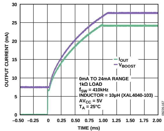
Figure 50. Output Current and V_{BOOST,x} Settling Time with DC-to-DC Converter (See Figure 81)
