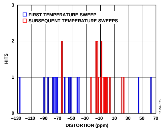
Figure 67. Thermal Hysteresis
