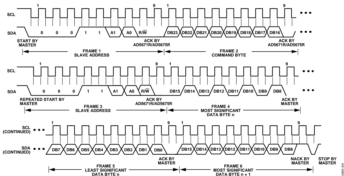
Figure 60. I 2 C Read Operation
