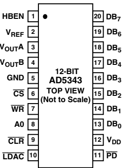
AD5343 PIN CONFIGURATION
