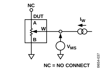
Figure 36. Resistor Position Nonlinearity Error (Rheostat Operation: R-INL, R-DNL)
