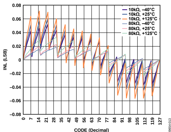
Figure 12. INL vs. Code (AD5111)
