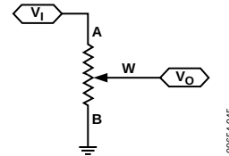
Figure 44. Potentiometer Mode Configuration
