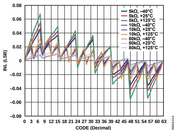
Figure 13. INL vs. Code (AD5113)
