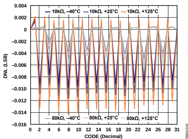
Figure 17. DNL vs. Code (AD5115)
