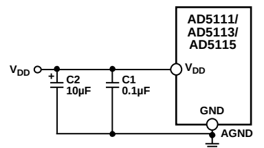
Figure 46. Power Supply Bypassing
