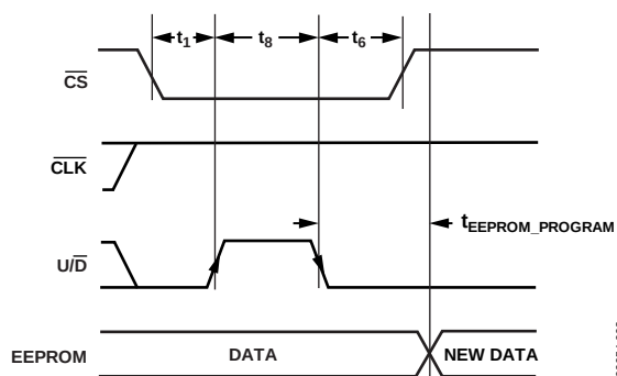
Figure 3. Storage Mode Timing
