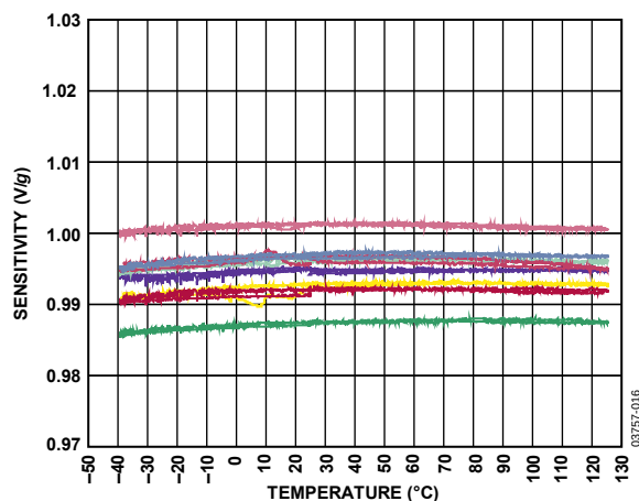
Figure 13. Sensitivity vs. Temperature; Devices Soldered to PCB
