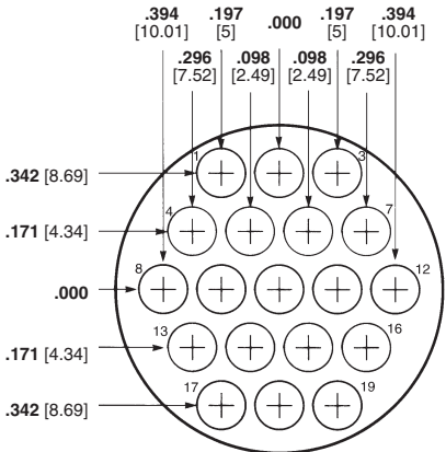
Arrangement 23-19 Max. Wire Ins. Dia. = .150 [3.81]
