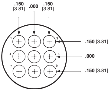
Arrangement 13-9 Max. Wire Ins. Dia. = .100 [2.54]
