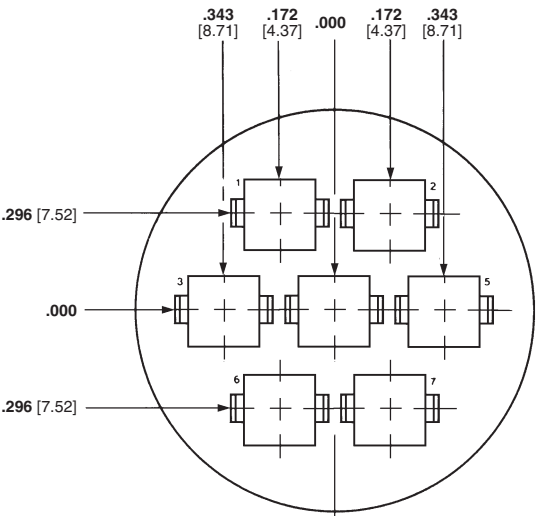
Shell Size 23
