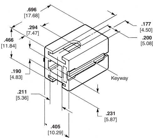
Wire-To-Wire Connector Housing
