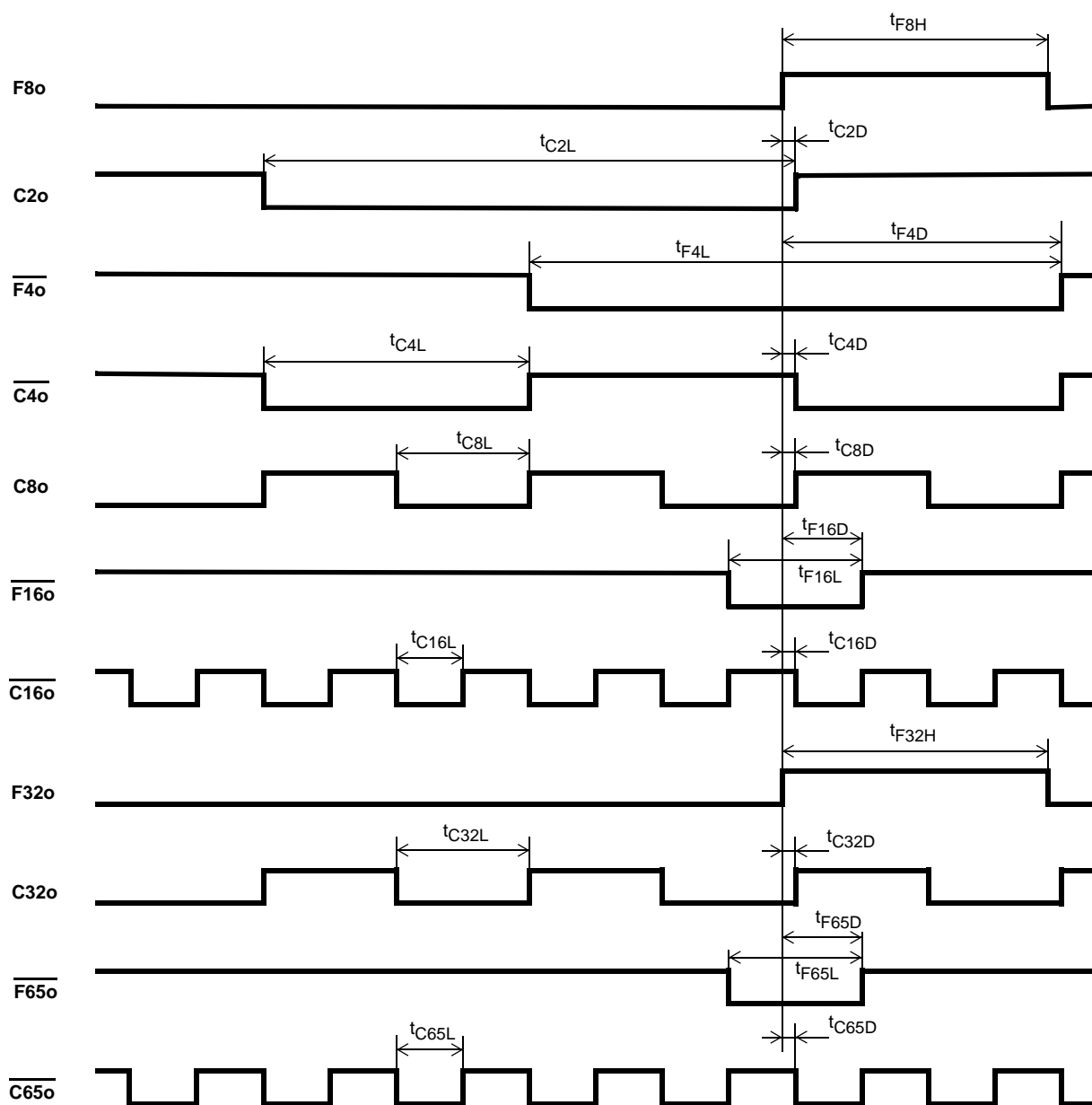
Figure 28 - E1 Output Timing Referenced to F8/F32o
