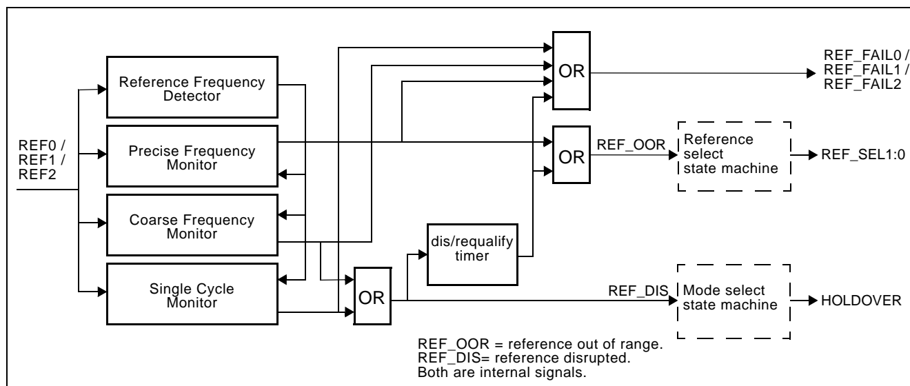
Figure 3 - Reference Monitor Circuit
