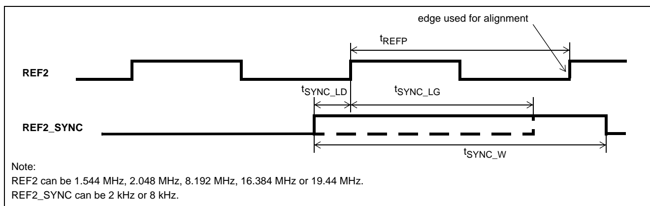
Figure 27 - REF2_SYNC Timing
