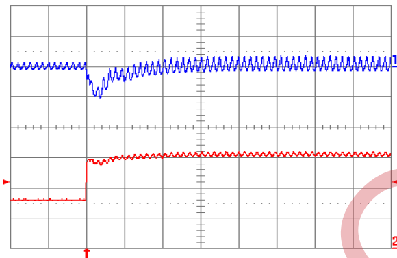
Fig. 1.0V.7: Output voltage response for V_{out} = 1.0\text{ V} to positive load current step change from 2.5 A to 5 A with slew rate of 5\text{ A}/\mu\text{s} at V_{in} = 5\text{ V} . Top trace: output voltage (100 mV/div.); Bottom trace: load current (2 A/div.). C_o = 47\text{ }\mu\text{F} ceramic + 1\text{ }\mu\text{F} ceramic. Time scale: 20 \mu\text{s} /div.
