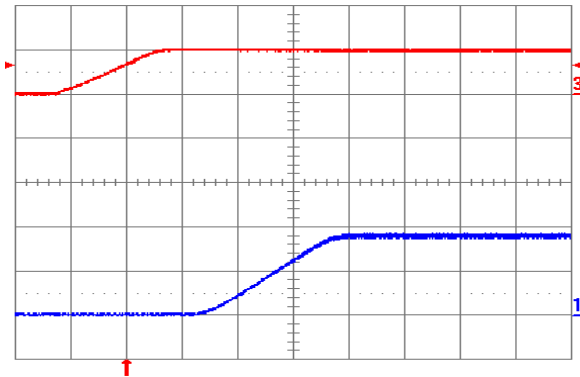
Fig. 1.8V.5: Turn-on transient for V_{out} = 1.8\text{ V} with application of V_{in} at full rated load current (resistive) and 47\text{ }\mu\text{F} external capacitance at V_{in} = 5\text{ V} . Top trace: V_{in} (5 V/div.); Bottom trace: output voltage (1 V/div.); Time scale: 2 ms/div.
