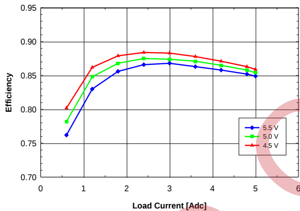
Fig. 1.2V.3: Efficiency vs. load current and input voltage for V_{out} = 1.2 V converter mounted vertically with air flowing from pin 5 to pin 1 at a rate of 200 LFM (1 m/s) and T_a = 25 °C.
