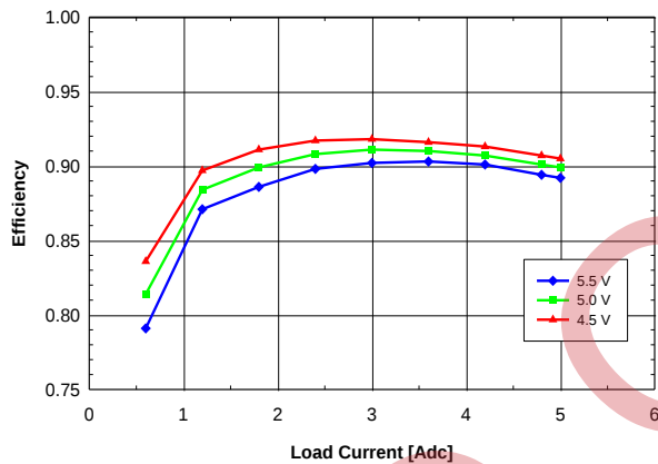
Fig. 2.0V.3: Efficiency vs. load current and input voltage for V_{out} = 2.0 V converter mounted vertically with air flowing from pin 5 to pin 1 at a rate of 200 LFM (1 m/s) and T_a = 25 °C.
