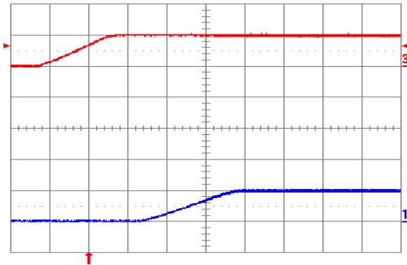
Fig. 1.0V.5: Turn-on transient for V_{out} = 1.0\text{ V} with application of V_{in} at full rated load current (resistive) and 47\text{ }\mu\text{F} external capacitance at V_{in} = 5\text{ V} . Top trace: V_{in} (5 V/div.); Bottom trace: output voltage (1 V/div.); Time scale: 2 ms/div.
