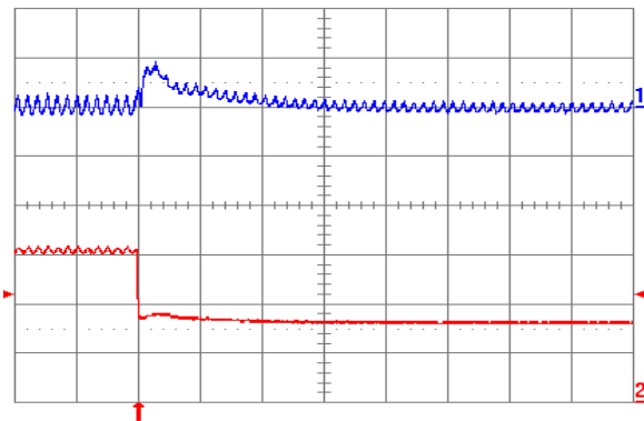
Fig. 0.7525V.8: Output voltage response for V_{out} = 0.7525 V to negative load current step change from 5 A to 2.5 A with slew rate of -5 A/ \mu s at V_{in} = 5 V. Top trace: output voltage (100 mV/div.); Bottom trace: load current (2 A/div.). C_o = 47 \mu F ceramic + 1 \mu F ceramic. Time scale: 20 \mu s/div.
