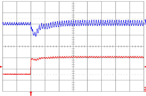
Fig. 1.2V.6: Output voltage response for V_{out} = 1.2\text{ V} to positive load current step change from 2.5\text{ A} to 5\text{ A} with slew rate of 5\text{ A}/\mu\text{s} at V_{in} = 5\text{ V} . Top trace: output voltage ( 100\text{ mV/div.} ); Bottom trace: load current ( 2\text{ A/div.} ). C_o = 47\text{ }\mu\text{F ceramic} + 1\text{ }\mu\text{F ceramic} . Time scale: 20\text{ }\mu\text{s/div.}
