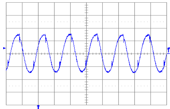
Fig. 2.0V.6: Output voltage ripple (20 mV/div.) at full rated load current into a resistive load with external capacitance 10 \mu\text{F} ceramic + 1 \mu\text{F} ceramic and V_{in} = 5 V for V_{out} = 2.0 V. Time scale: 2 μs/div.
