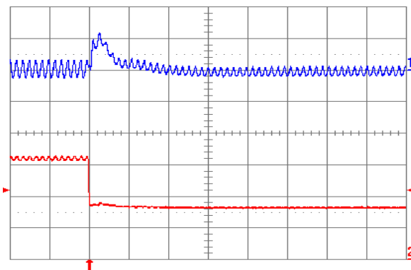
Fig. 1.5V.8: Output voltage response for V_{out} = 1.5 V to negative load current step change from 5 A to 2.5 A with slew rate of -5 A/ \mu s at V_{in} = 5 V. Top trace: output voltage (100 mV/div.); Bottom trace: load current (2 A/div.). C_o = 47 \mu F ceramic + 1 \mu F ceramic. Time scale: 20 \mu s/div.
