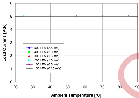
Fig. 1.8V.1: Available load current vs. ambient temperature and airflow rates for V_{out} = 1.8\text{ V} converter mounted vertically with V_{in} = 5\text{ V} , air flowing from pin 5 to pin 1, and maximum MOSFET temperature \leq 120\text{ }^{\circ}\text{C} .
