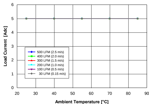
Fig. 1.5V.2: Available load current vs. ambient temperature and airflow rates for V_{out} = 1.5\text{ V} converter mounted horizontally with V_{in} = 5\text{ V} , air flowing from pin 5 to pin 1, and maximum MOSFET temperature \leq 120\text{ }^{\circ}\text{C} .
