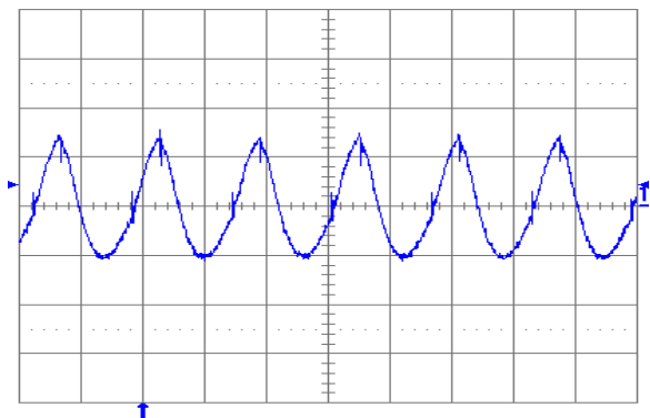
Fig. 1.2V.6: Output voltage ripple (20 mV/div.) at full rated load current into a resistive load with external capacitance 10 \mu\text{F} ceramic + 1 \mu\text{F} ceramic and V_{in} = 5 V for V_{out} = 1.2 V. Time scale: 2 μs/div.
