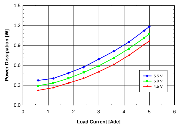
Fig. 3.3V.4: Power Loss vs. load current and input voltage for V_{out} = 3.3\text{ V} converter mounted vertically with air flowing from pin 5 to pin 1 at a rate of 200 LFM (1 m/s) and T_a = 25^\circ\text{C} .
