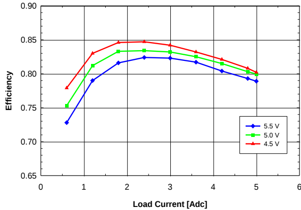
Fig. 0.7525V.3: Efficiency vs. load current and input voltage for V_{out} = 0.7525 V converter mounted vertically with air flowing from pin 5 to pin 1 at a rate of 200 LFM (1 m/s) and T_a = 25 °C.
