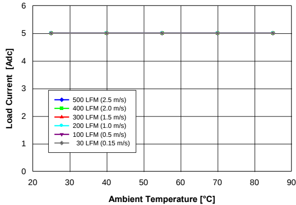
Fig. 2.0V.1: Available load current vs. ambient temperature and airflow rates for V_{out} = 2.0 V converter mounted vertically with V_{in} = 5 V, air flowing from pin 5 to pin 1, and maximum MOSFET temperature \leq 120 °C.
