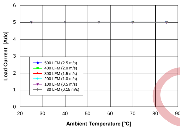
Fig. 3.3V.1: Available load current vs. ambient temperature and airflow rates for V_{out} = 3.3\text{ V} converter mounted vertically with V_{in} = 5\text{ V} , air flowing from pin 5 to pin 1, and maximum MOSFET temperature \leq 120^\circ\text{C} .
