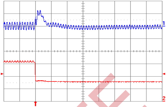
Fig. 2.0V.8: Output voltage response for V_{out} = 2.0\text{ V} to negative load current step change from 5\text{ A} to 2.5\text{ A} with slew rate of -5\text{ A}/\mu\text{s} at V_{in} = 5\text{ V} . Top trace: output voltage ( 100\text{ mV}/\text{div.} ); Bottom trace: load current ( 2\text{ A}/\text{div.} ). C_o = 47\text{ }\mu\text{F} ceramic + 1\text{ }\mu\text{F} ceramic. Time scale: 20\text{ }\mu\text{s}/\text{div.}
