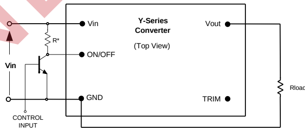
Fig. C: Circuit configuration for ON/OFF function.
