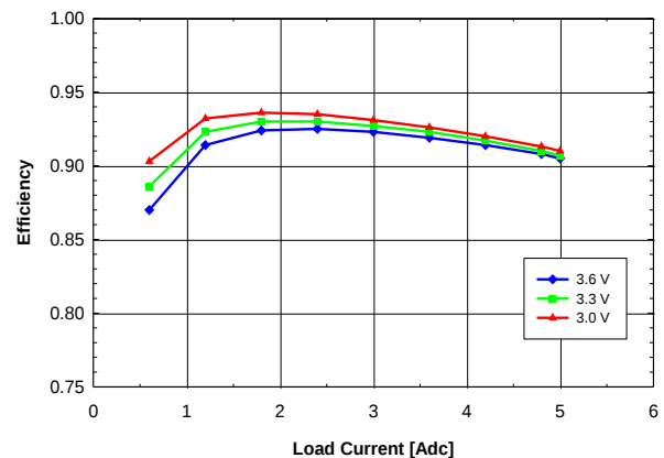
Fig. 1.8V.4: Efficiency vs. load current and input voltage for V_{out} = 1.8\text{ V} converter mounted vertically with air flowing from pin 5 to pin 1 at a rate of 200\text{ LFM} ( 1\text{ m/s} ) and T_a = 25\text{ }^{\circ}\text{C} .
