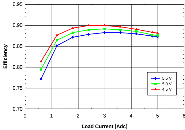
Fig. 1.5V.3: Efficiency vs. load current and input voltage for V_{out} = 1.5 V converter mounted vertically with air flowing from pin 5 to pin 1 at a rate of 200 LFM (1 m/s) and T_a = 25 °C.
