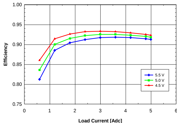
Fig. 2.5V.3: Efficiency vs. load current and input voltage for V_{out} = 2.5 V converter mounted vertically with air flowing from pin 5 to pin 1 at a rate of 200 LFM (1 m/s) and T_a = 25 °C.
