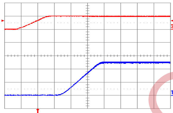
Fig. 2.5V.4: Turn-on transient for V_{out} = 2.5 V with application of V_{in} at full rated load current (resistive) and 47 \mu F external capacitance at V_{in} = 5 V. Top trace: V_{in} (5 V/div.); Bottom trace: output voltage (1V/div.); Time scale: 2 ms/div.
