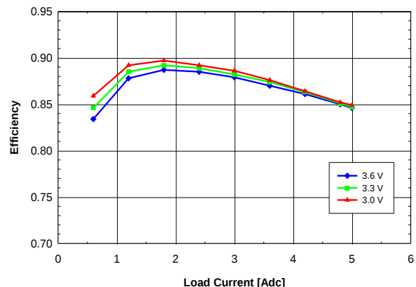
Fig. 1.0V.4: Efficiency vs. load current and input voltage for V_{out} = 1.0\text{ V} converter mounted vertically with air flowing from pin 5 to pin 1 at a rate of 200\text{ LFM} ( 1\text{ m/s} ) and T_a = 25\text{ }^{\circ}\text{C} .
