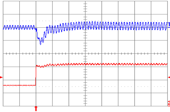
Fig. 2.0V.7: Output voltage response for V_{out} = 2.0\text{ V} to positive load current step change from 2.5\text{ A} to 5\text{ A} with slew rate of 5\text{ A}/\mu\text{s} at V_{in} = 5\text{ V} . Top trace: output voltage ( 100\text{ mV}/\text{div.} ); Bottom trace: load current ( 2\text{ A}/\text{div.} ). C_o = 47\text{ }\mu\text{F} ceramic + 1\text{ }\mu\text{F} ceramic. Time scale: 20\text{ }\mu\text{s}/\text{div.}
