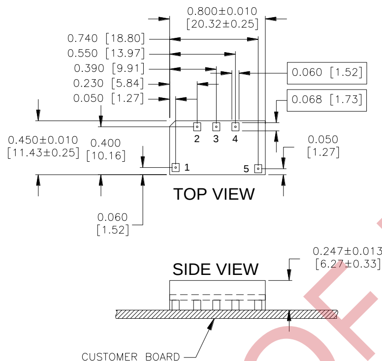
YNM05S Pinout (Surface Mount)
