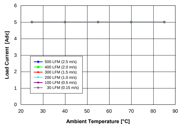
Fig. 2.5V.2: Available load current vs. ambient temperature and airflow rates for V_{out} = 2.5\text{ V} converter mounted horizontally with V_{in} = 5\text{ V} , air flowing from pin 5 to pin 1, and maximum MOSFET temperature \leq 120\text{ }^{\circ}\text{C} .
