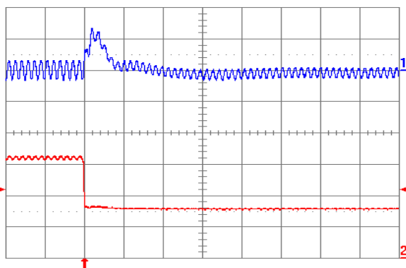
Fig. 2.5V.8: Output voltage response for V_{out} = 2.5 V to negative load current step change from 5 A to 2.5 A with slew rate of -5 A/ \mu s at V_{in} = 5 V. Top trace: output voltage (100 mV/div.); Bottom trace: load current (2 A/div.). C_o = 47 \mu F ceramic + 1 \mu F ceramic. Time scale: 20 \mu s/div.
