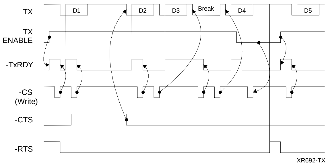
Figure 9: Transmit Timing
