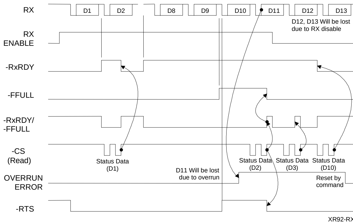
Figure 8: Receive Timing
