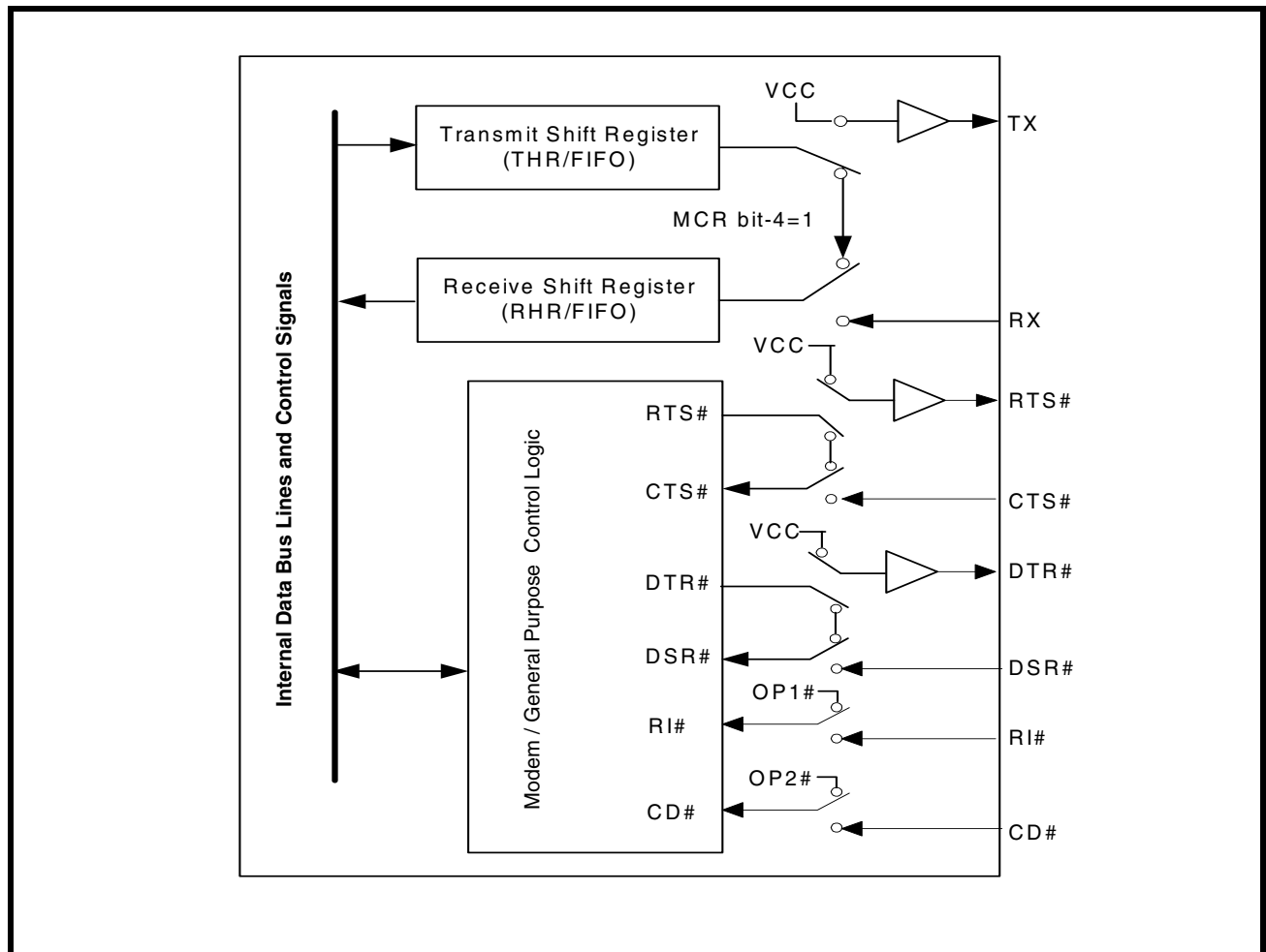
FIGURE 15. INTERNAL LOOPBACK
