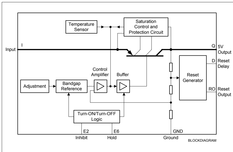
Figure 3 Block Diagram
