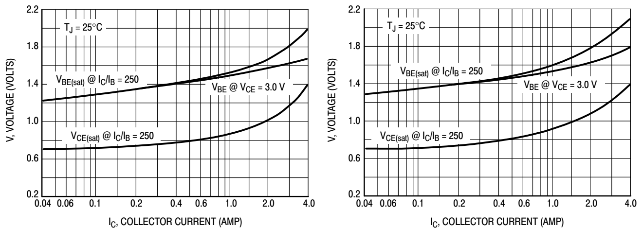
Figure 11. "On" Voltages
