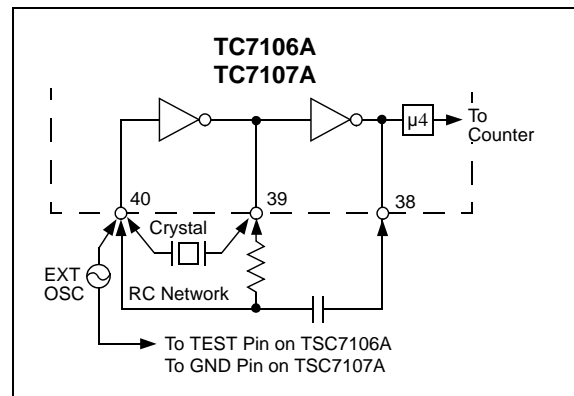
FIGURE 6-1: Clock Circuits.
