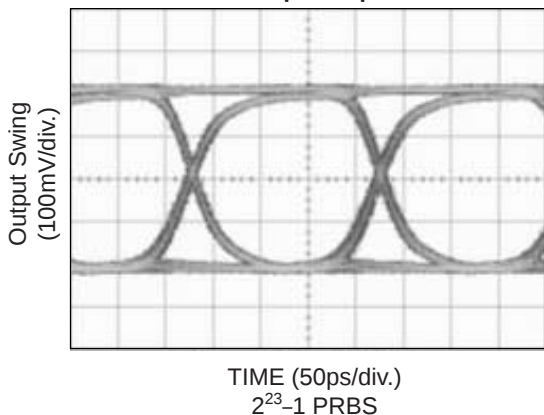
10.7Gbps Output
