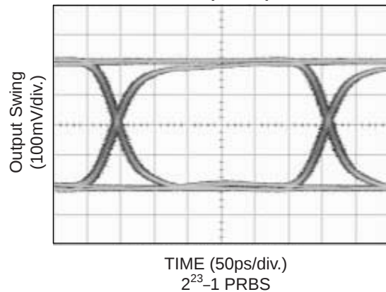
3.2Gbps Output
