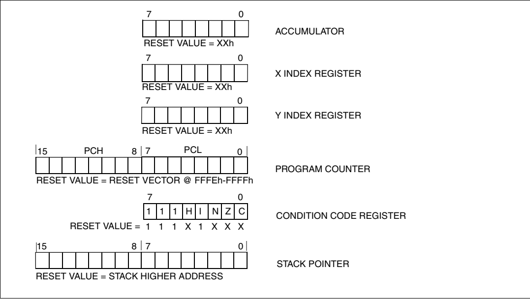
Figure 11. CPU registers
