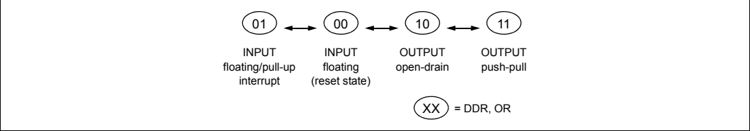
Figure 33. Interrupt I/O port state transitions
