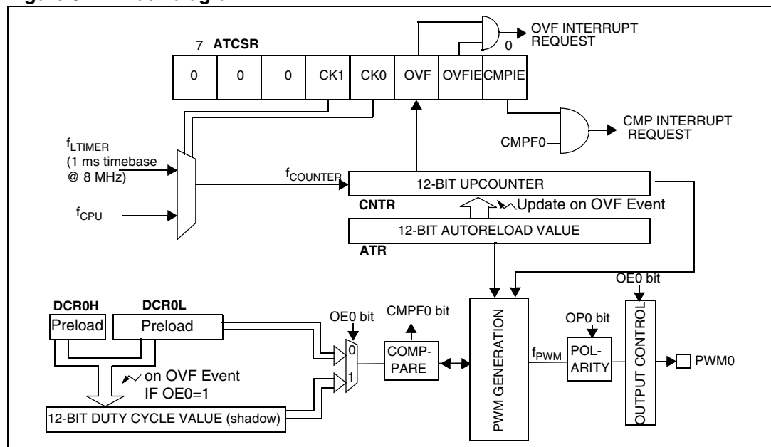
Figure 37. Block diagram
