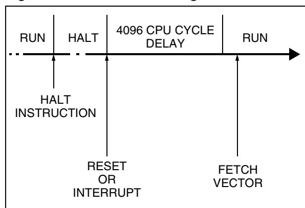
Figure 25. HALT Mode Timing Overview
