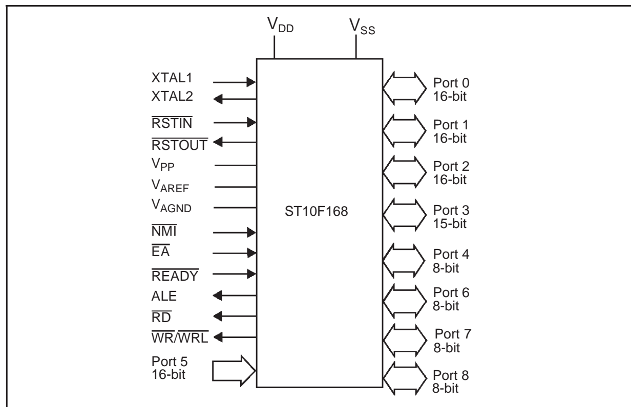
Figure 1 : Logic Symbol
