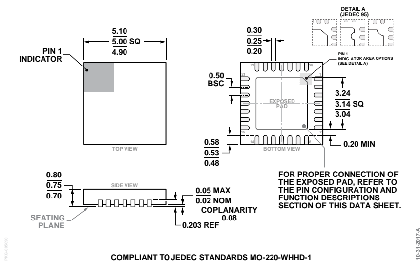
COMPLIANT TO JEDEC STANDARDS MO-220-WHHD-1 Figure 32. 28-Lead Lead Frame Chip Scale Package [LFCSP] 5 mm x 5 mm Body and 0.75 mm Package Height (CP-28-10) Dimensions shown in millimeters
