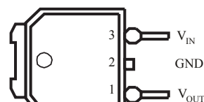
TO-252 (R)
