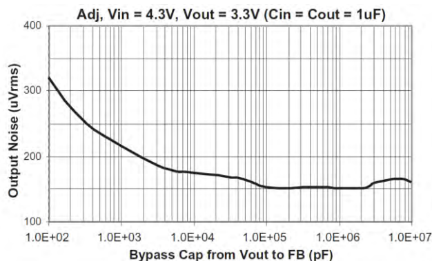
Fig. 42: Noise Performance 10Hz to 100kHz
