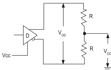
Figure 1: Driver DC Test Load Circuit
