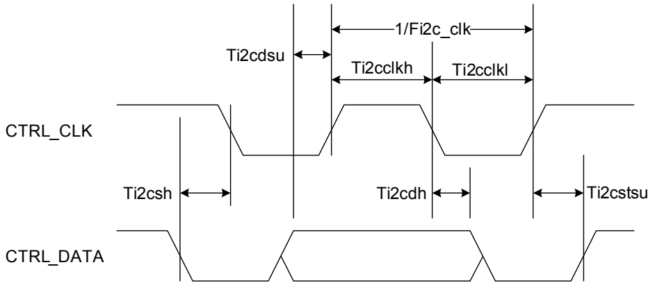
Figure 5. I 2 C Timing (CTRL_MODE == 0)
