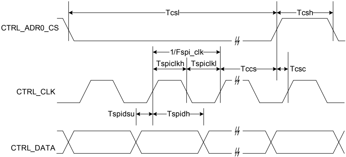
Figure 6. SPI Timing
