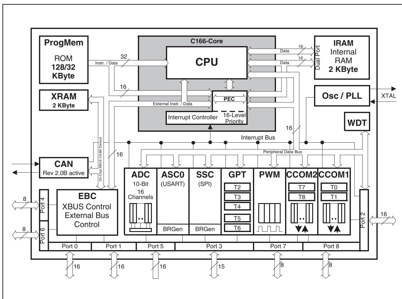
Figure 4 Block Diagram
