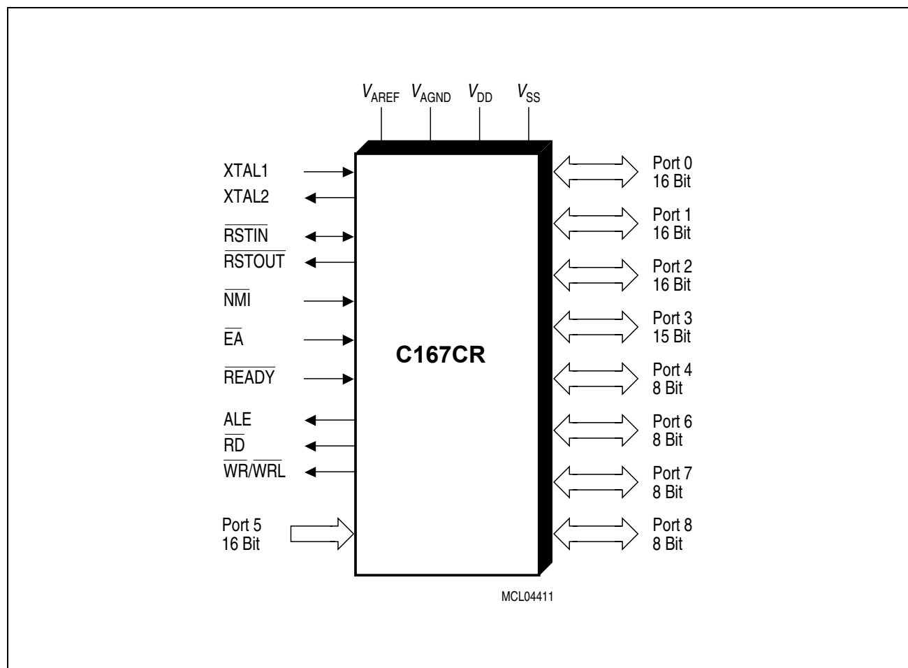
Figure 1 Logic Symbol
