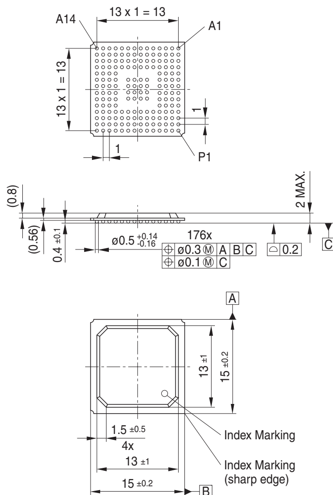
Figure 25 P-BGA-176-2 (Plastic Ball Grid Array Package)
