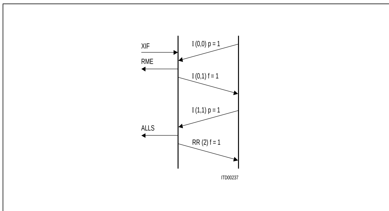
Figure 17 Data Reception/Transmission
