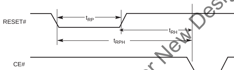
Figure 20.1 Reset Timings
