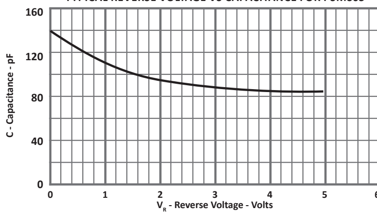
FIGURE 5 TYPICAL REVERSE VOLTAGE VS CAPACITANCE FOR PSMS05
