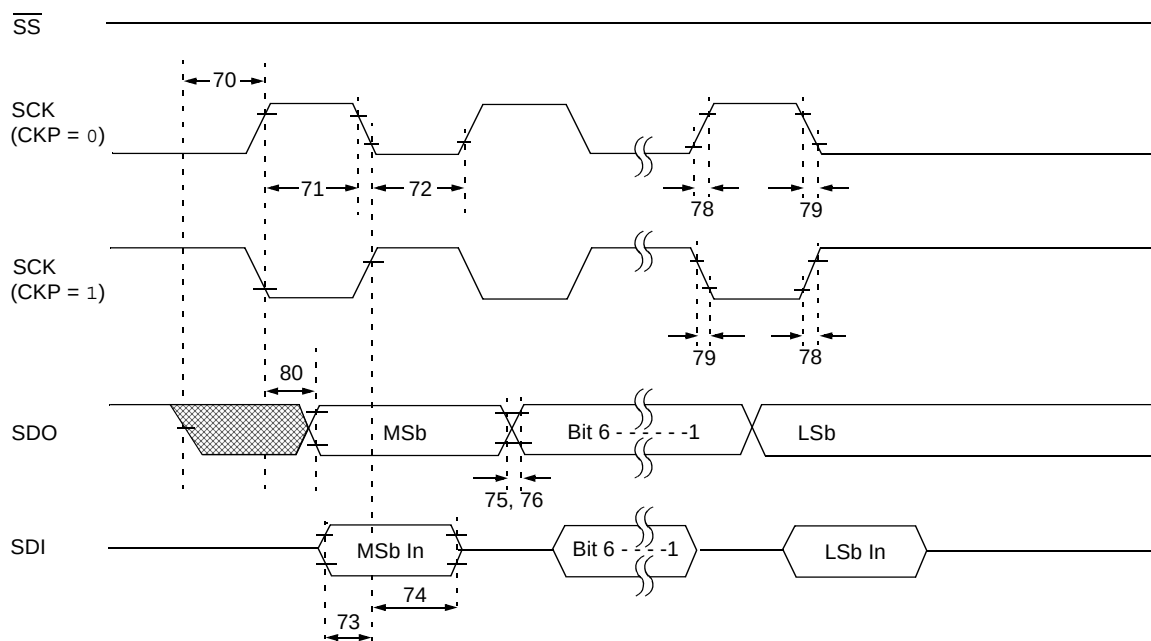
FIGURE 15-10: SPI™ MASTER MODE TIMING (CKE = 0, SMP = 0)
