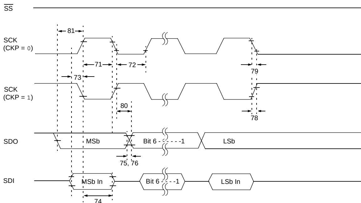
FIGURE 15-11: SPI™ MASTER MODE TIMING (CKE = 1, SMP = 1)
