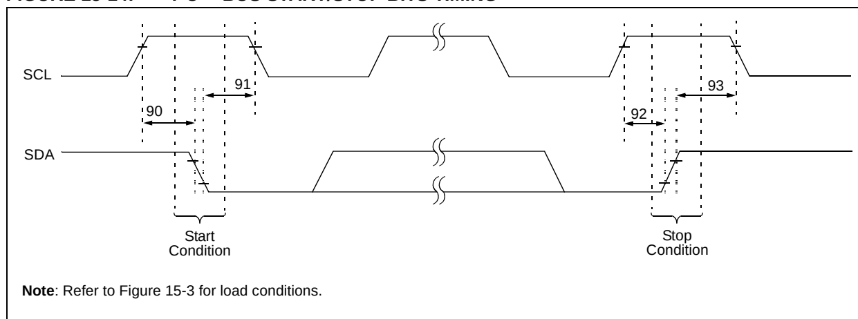
FIGURE 15-14: I²C™ BUS START/STOP BITS TIMING
