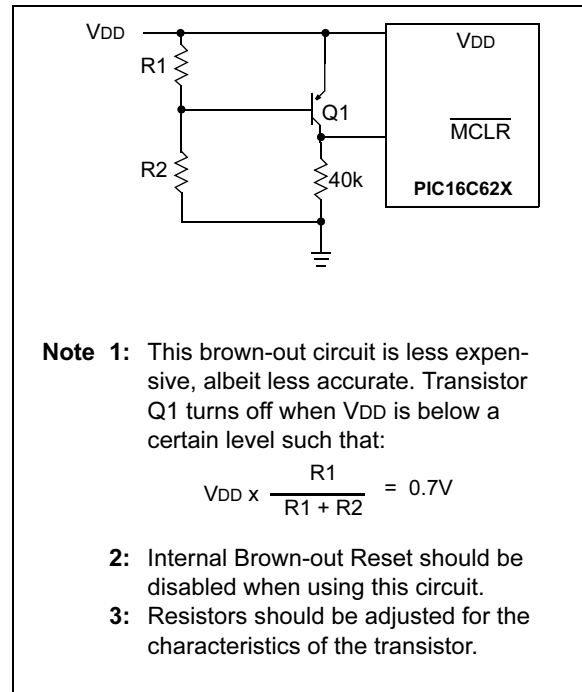
FIGURE 9-13: EXTERNAL BROWN-OUT PROTECTION CIRCUIT 2
