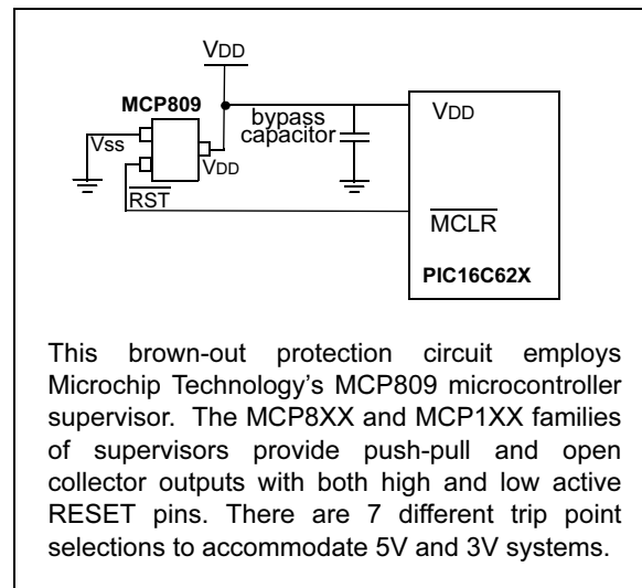
FIGURE 9-14: EXTERNAL BROWN-OUT PROTECTION CIRCUIT 3
