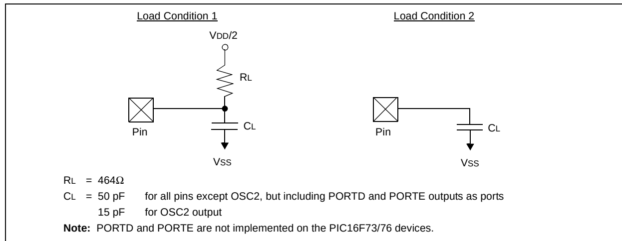
FIGURE 15-3: LOAD CONDITIONS
