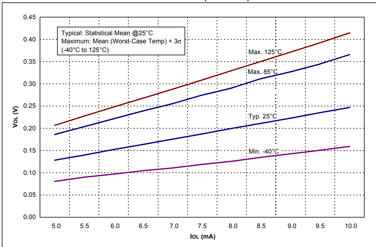
FIGURE 14-9: V_{OL} vs. I_{OL} OVER TEMPERATURE ( V_{DD} = 5.0V )
