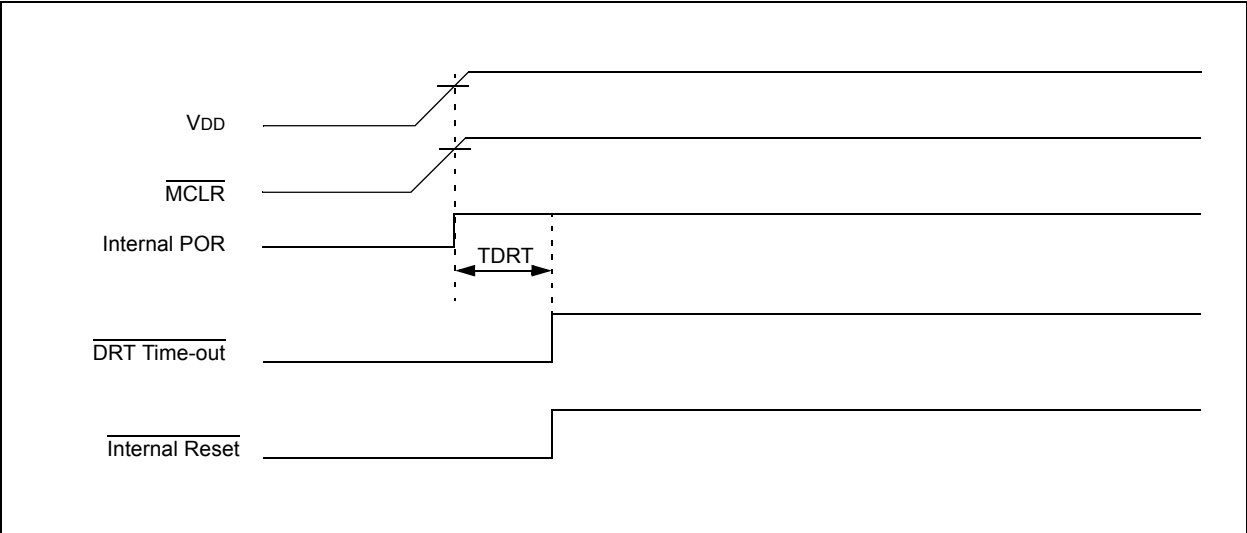
FIGURE 10-9: TIME-OUT SEQUENCE ON POWER-UP ( \overline{\text{MCLR}} TIED TO \text{V}_{\text{DD}} ): FAST \text{V}_{\text{DD}} RISE TIME
