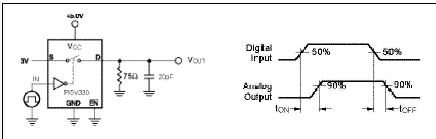
Figure 4. Switching Time
