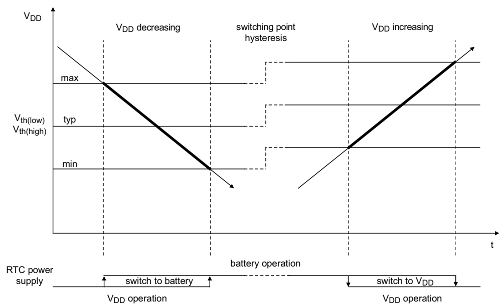
Fig 23. Threshold voltage switching hysteresis
