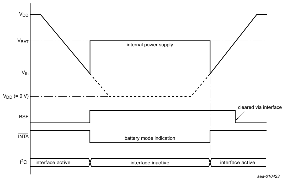
Fig 24. Switching at V_{th}
