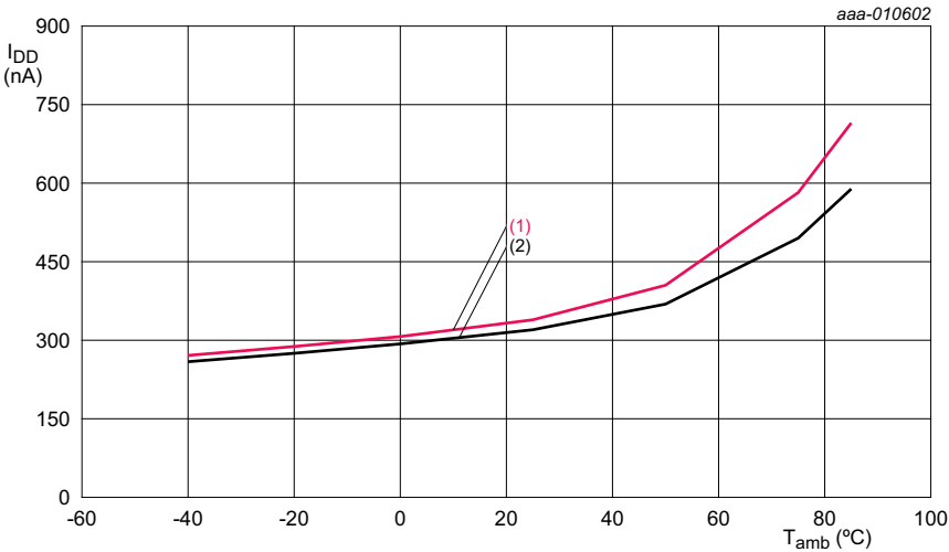
C L(itg) = 7 pF; CLKOUT disabled; battery switched on. (1) V DD = 5 V. (2) V DD = 3.3 V.
