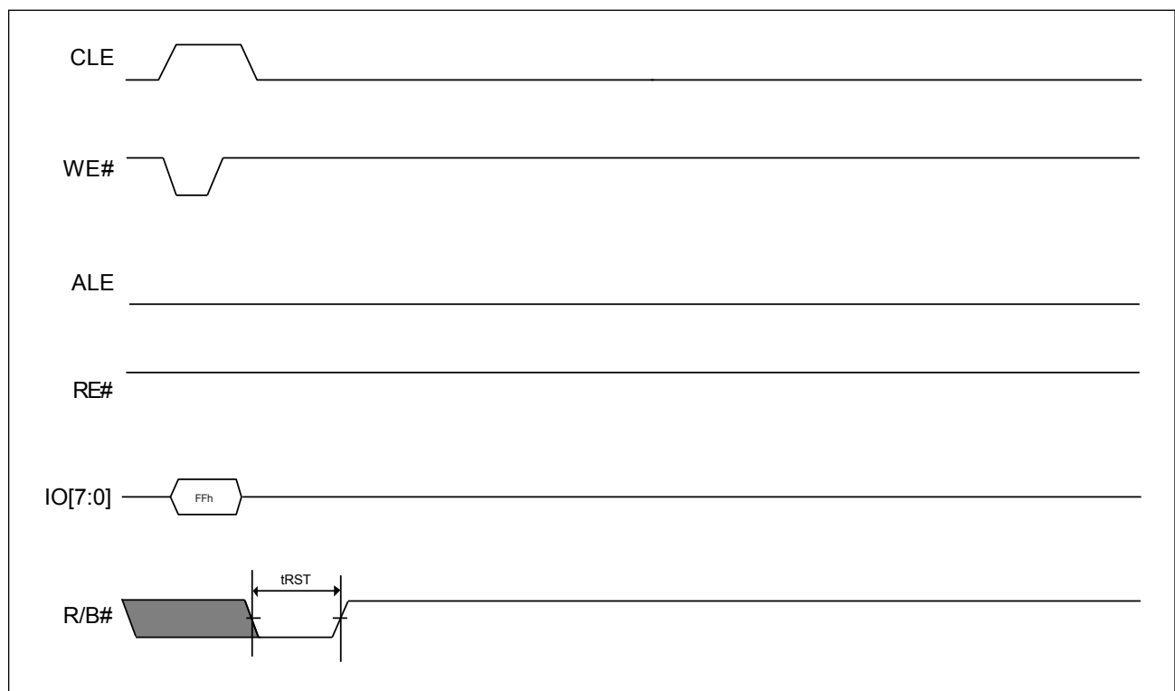
Figure 19. Reset Operation
