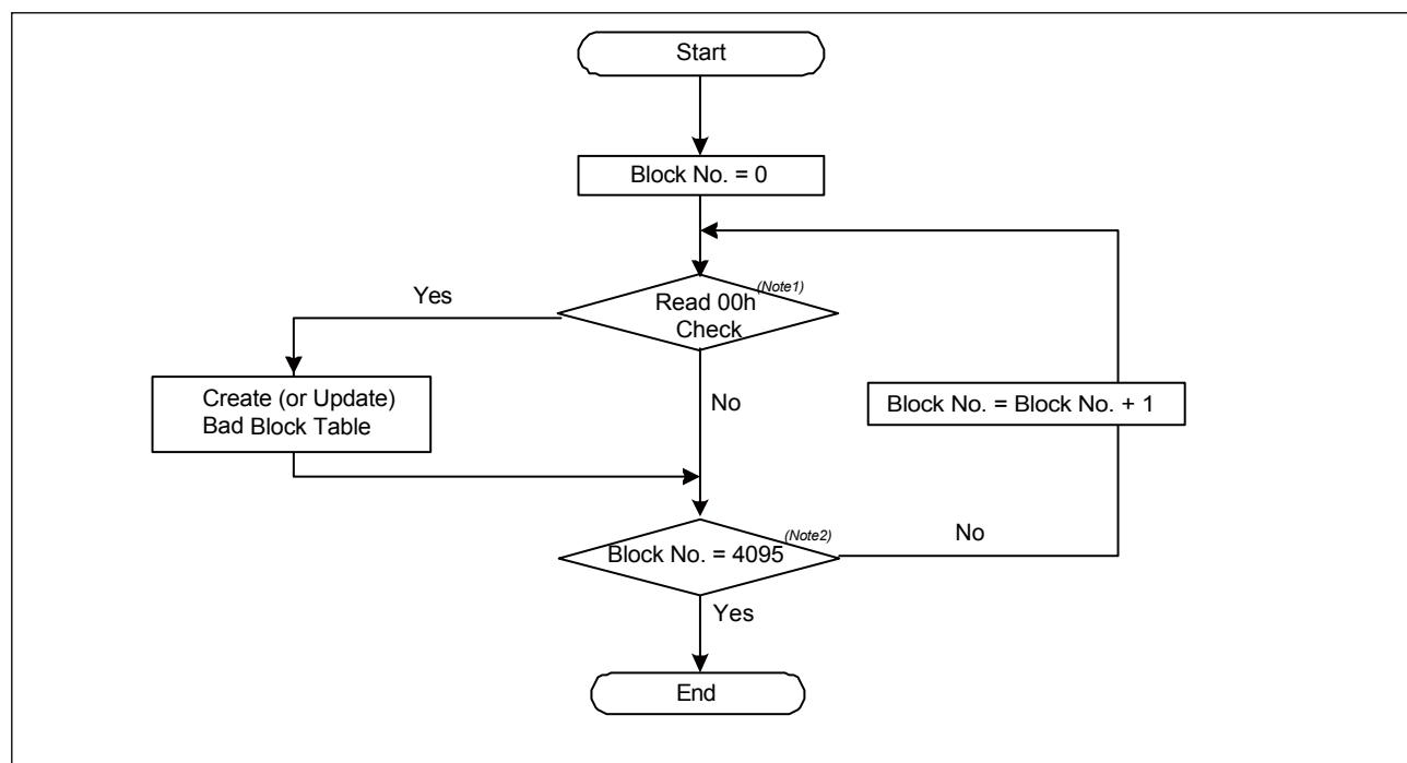
Figure 48. Bad Block Test Flow
