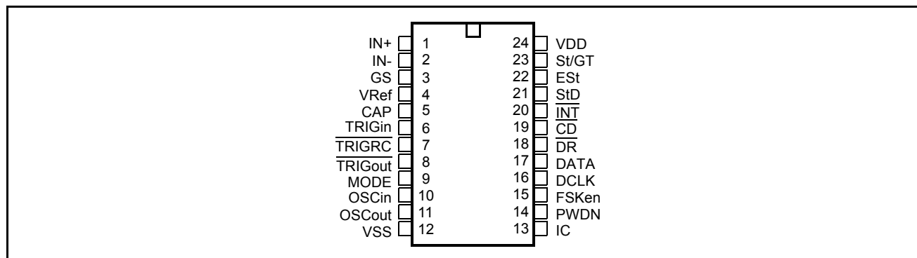
Figure 2 - Pin Connections
