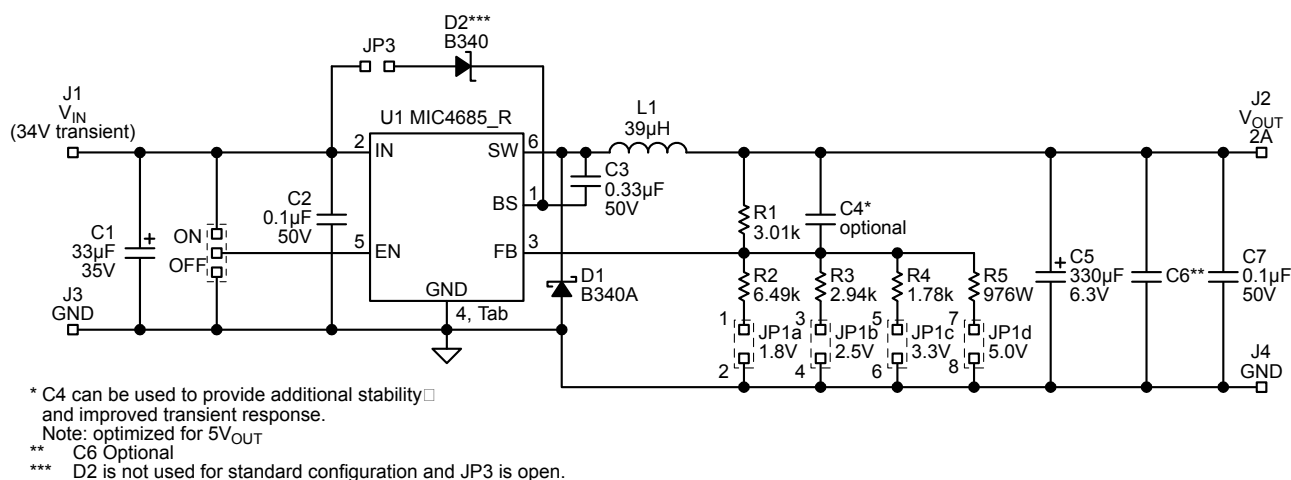
Figure 4. Evaluation Board Schematic Diagram
