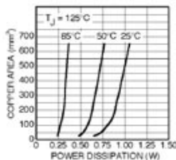
Figure 5. Copper Area vs. Power-MSOP Power Dissipation ( T_J )
