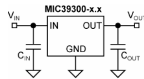
Figure 1. Capacitor Requirements
