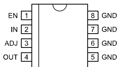
MIC3775 (Adjustable) 8-Pin MSOP (MM)
