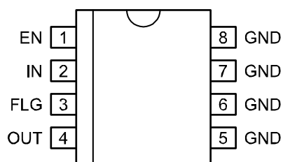
MIC3775-x.x (Fixed) 8-Pin MSOP (MM)
