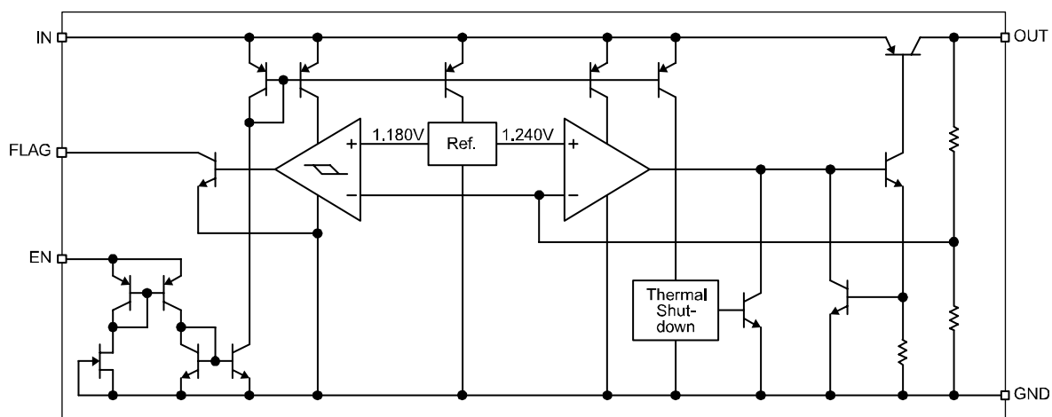
MIC3775 Fixed Regulator with Flag and Enable Block Diagram
