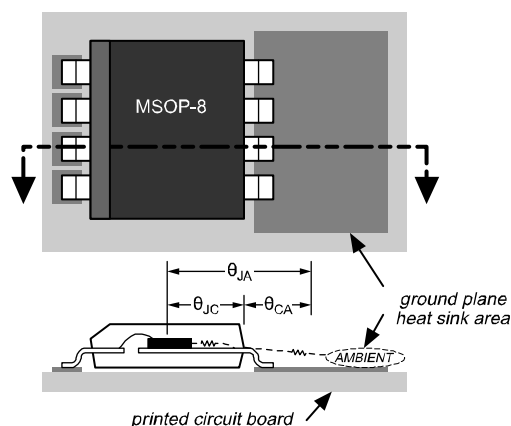
Figure 3. Thermal Resistance
