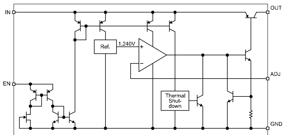
MIC3775 Adjustable Regulator Block Diagram
